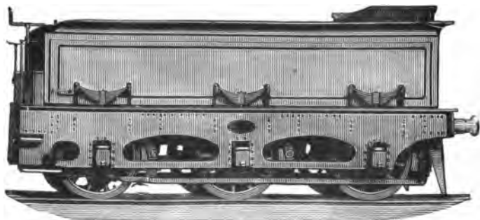
Fig. 74.—Midland Tender, No. 1631.
